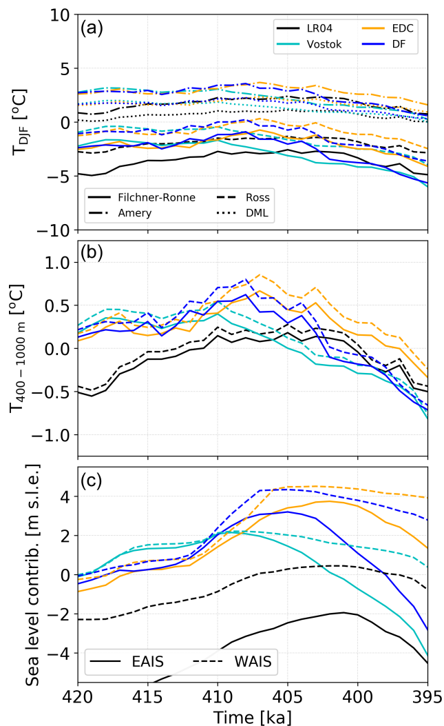
Figure 9. Evolution throughout MIS11c for each CFEN member for (a) summer surface air temperature [ ^{\circ}\text{C} ] averaged over the main Antarctic ice shelves, (b) ocean temperatures averaged between 400 and 1000 m [ ^{\circ}\text{C} ] for the Filchner–Ronne and Ross ice shelves, and (c) sea level contribution by EAIS and WAIS. Colours denote the respective CFEN member, while line styles in panels (a) and (b) denote each ice shelf and each ice sheet in panel (c). DML refers to all smaller ice shelves along the Dronning Maud Land margin.
