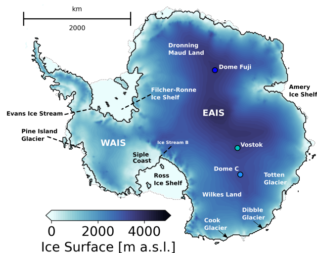
Figure 1. Surface topography of the AIS at the start of our core experiments (425 ka), based on a calibration against Bedmap2, (Fretwell et al., 2013, see Sect. 2.1). Locations mentioned in the text are showcased, including the drilling sites of the ice cores used in this study (circles).
