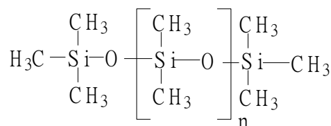
Figur 1 Dimetylpolysilan
