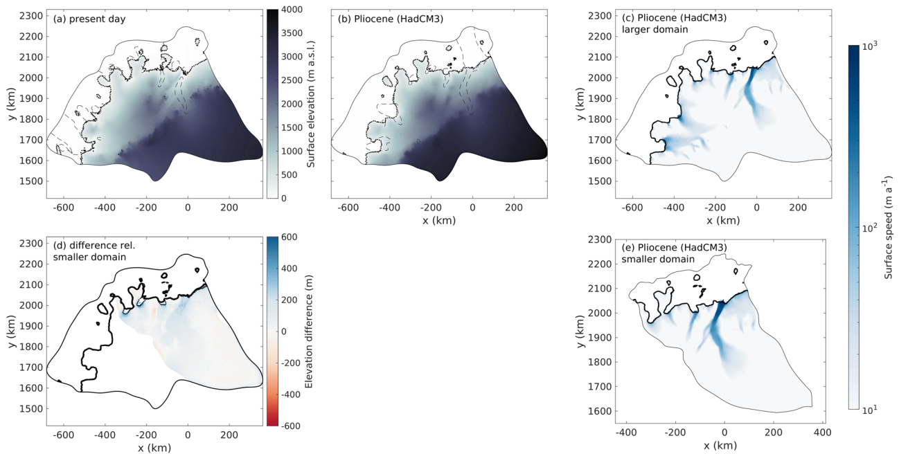
Fig. 4 Showcase of the lower-resolution, larger-domain experiment. a Modern surface topography (m a.s.l.). b Pliocene surface topography (the difference between both is presented in Fig. 3a). c Pliocene surface speed ( \text{ma}^{-1} ). d Pliocene ice-surface elevation difference (m) between the larger-domain and the smaller-domain experiments (blue means the larger domain produces higher elevations). e Pliocene surface speed for the smaller domain, for comparison with panel (c). Dashed lines in panels a , b denote the 50 \text{ ma}^{-1} surface speed contour, while solid lines in all panels show the grounding line. In summary, the larger experiment yields a thicker Jutulstraumen, while Schyttbreen loses less mass due to ice advection from the western part of the domain. This increased mass advection, however, is not enough to significantly counter the effects of dynamic thinning at Schyttbreen or the other smaller glaciers.
