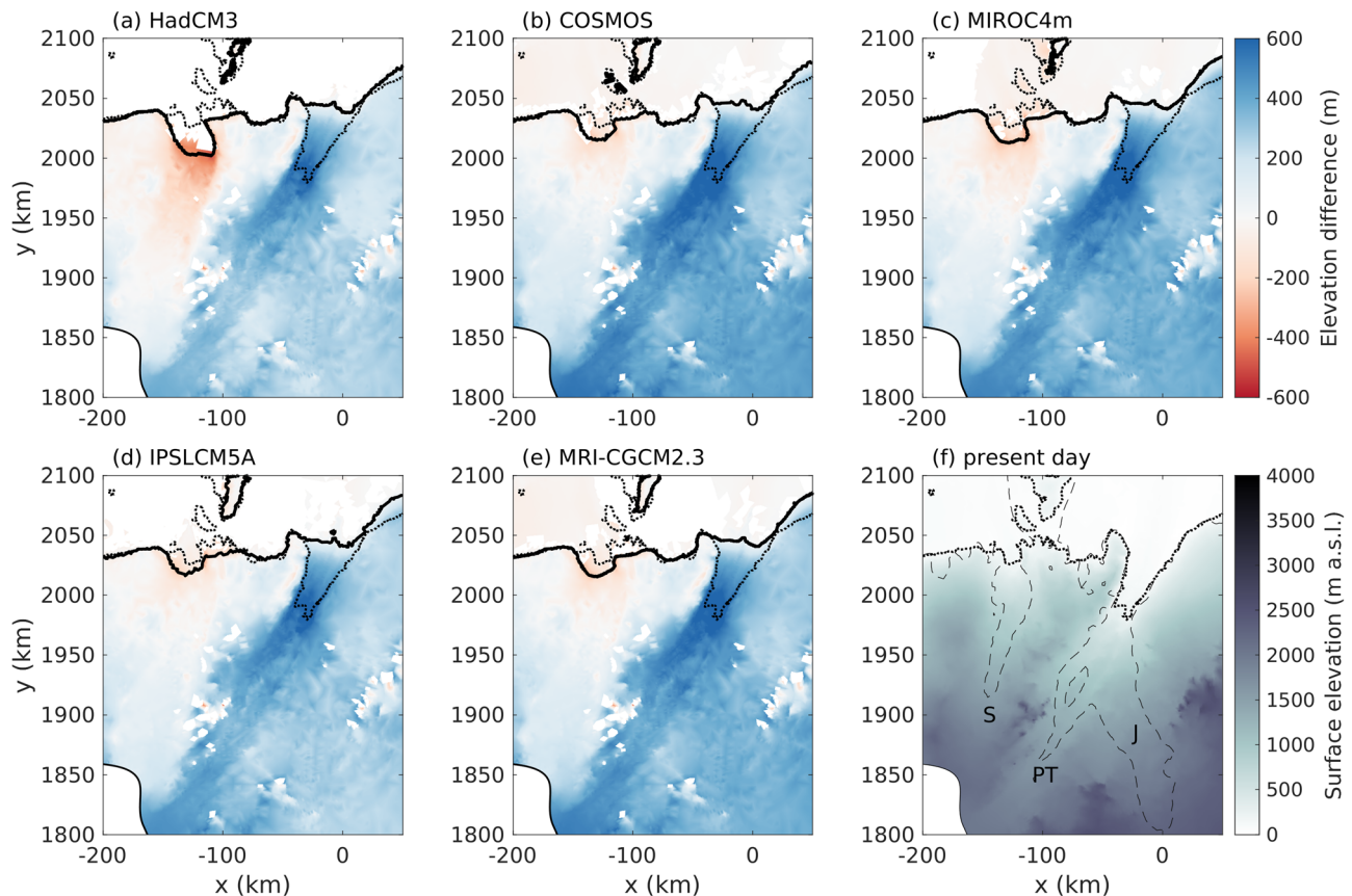
Fig. 2 Jutulstraumen is thicker under all climate forcings. a–e Ice-surface elevation differences between all Pliocene-forced experiments and present day 23 (panel f). Panel (f) also shows the 50 \text{m s}^{-1} surface speed contour as dashed grey lines, highlighting the ice streams, which are marked with S (Schyttbreen), PT (Penck Trough), and J (Jutulstraumen). Black dashed lines in all panels show the modern grounding-line position, while black solid lines show the modelled Pliocene position.
