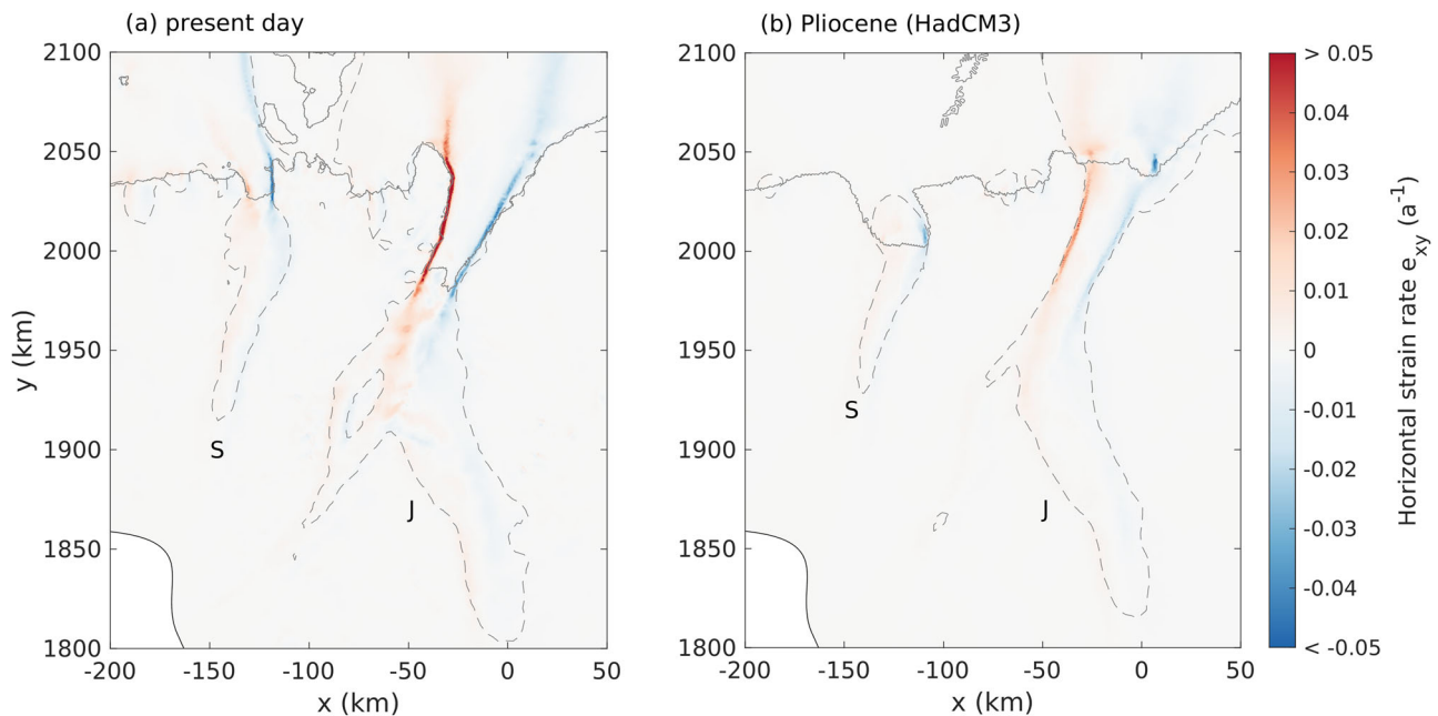
Fig. 6 Lateral stresses are significantly higher along the Jutulstraumen flux gate. Horizontal strain rates ( \text{a}^{-1} ) for a the modern ice sheet and b the Pliocene ice sheet. The solid line shows the grounding line position and the dashed lines show the 50 \text{ m a}^{-1} surface speed contour. Schyttbreen and Jutulstraumen are identified by their initials.
