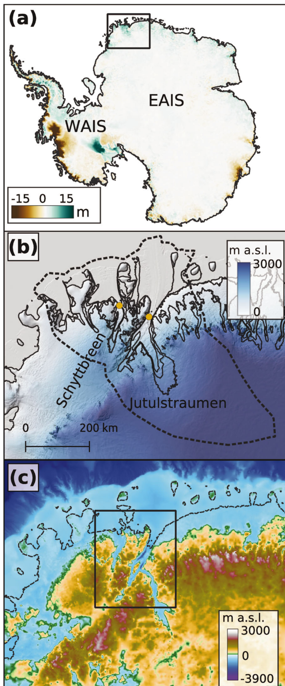
Fig. 1 Overview of DML and Jutulstraumen. a Grounded ice elevation changes between January 1994 and December 2020 from ITS_LIVE 84 , black rectangle highlights the DML area displayed in panels (b, c) ; WAIS and EAIS stand for West and East Antarctic Ice Sheet, respectively. b Contemporary ice-surface elevation (colours) 23 and ice surface speed contours 65 (solid lines denoting 20, 50, and 100 \text{ma}^{-1} increasing towards the margins). Shading highlights the steep topographic gradient between the ice sheet interior and the margin. Yellow dots mark the flux gates where elevation changes in Fig. 7 were computed. A thick dashed line marks the modelled domain, and a thin solid line shows the modern grounding line. c Modern subglacial topography 23 , including an updated dataset for Jutulstraumen 36 ; black rectangle highlights the area shown in Figs. 2 and 6 (smaller-domain experiments) while Fig. 3 (larger-domain experiment) covers the full extent of panel c . The thin dashed line marks the modern grounding line.
